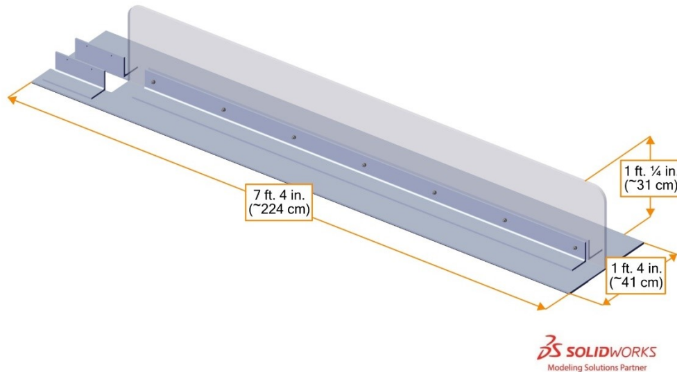
Figure 5-8: BARRIER
